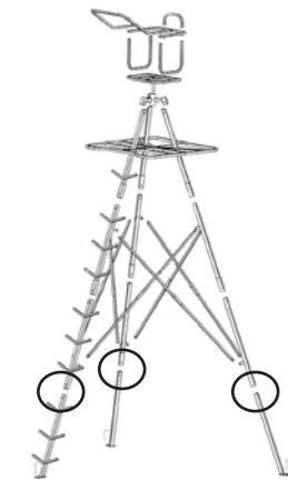
FIGURE 20 INSTALL LOWER LADDER SECTION AND LOWER LEGS
