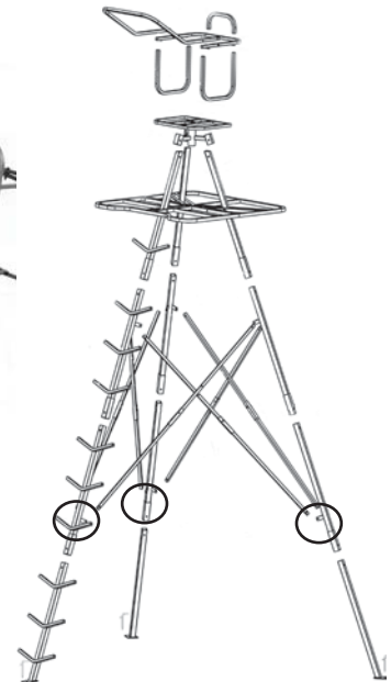
FIGURE 19 INSTALL CROSS BRACES AS SHOWN
