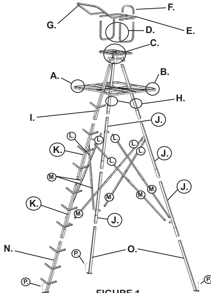
FIGURE 1 COMPONENTS OF OL' TIMER LADDER/DELUXE
