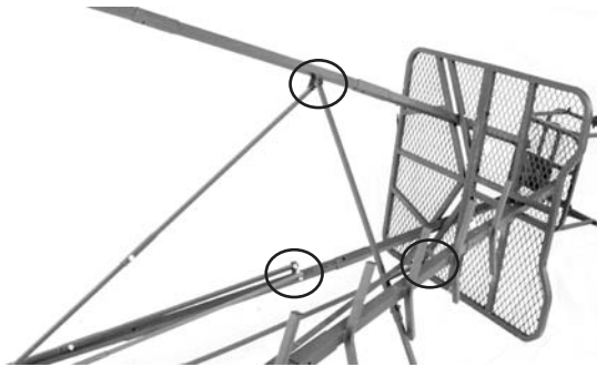
FIGURE 18 CROSS BRACES IN- STALLED ON UPPERMOST BRACKETS
