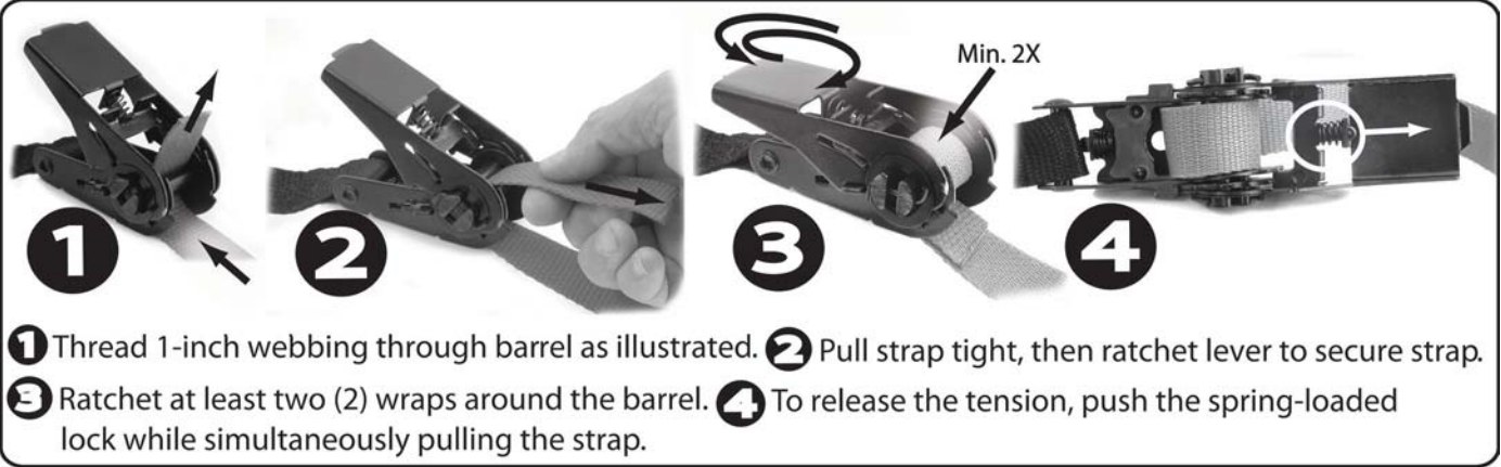
FIGURE 12 THREADING RATCHET STRAPS
