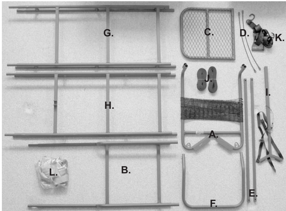
FIGURE 1 COMPONENTS OF OL' TIMER LADDER
